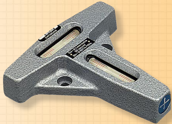
▲ Cross Spirit Level No. 52-422-079 Other sizes and sensitivities available upon request.
